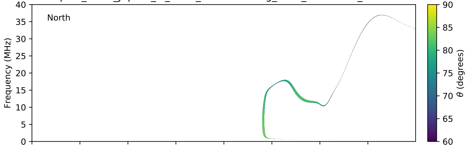
expres_earth_jupiter_io_isaac_lossc-wid1deg_3kev_20070411_v01.cdf
