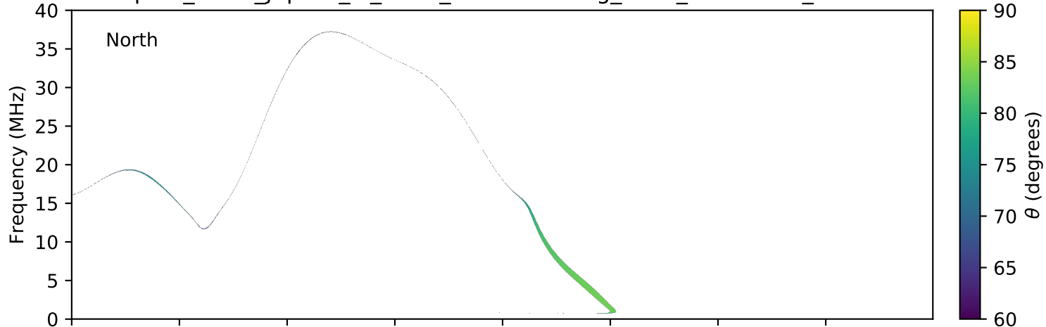
expres_earth_jupiter_io_isaac_lossc-wid1deg_3kev_20070410_v01.cdf
