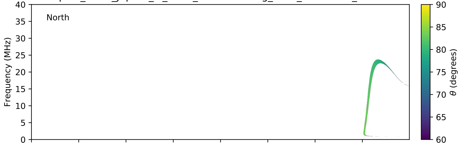
expres_earth_jupiter_io_isaac_lossc-wid1deg_3kev_20070409_v01.cdf
