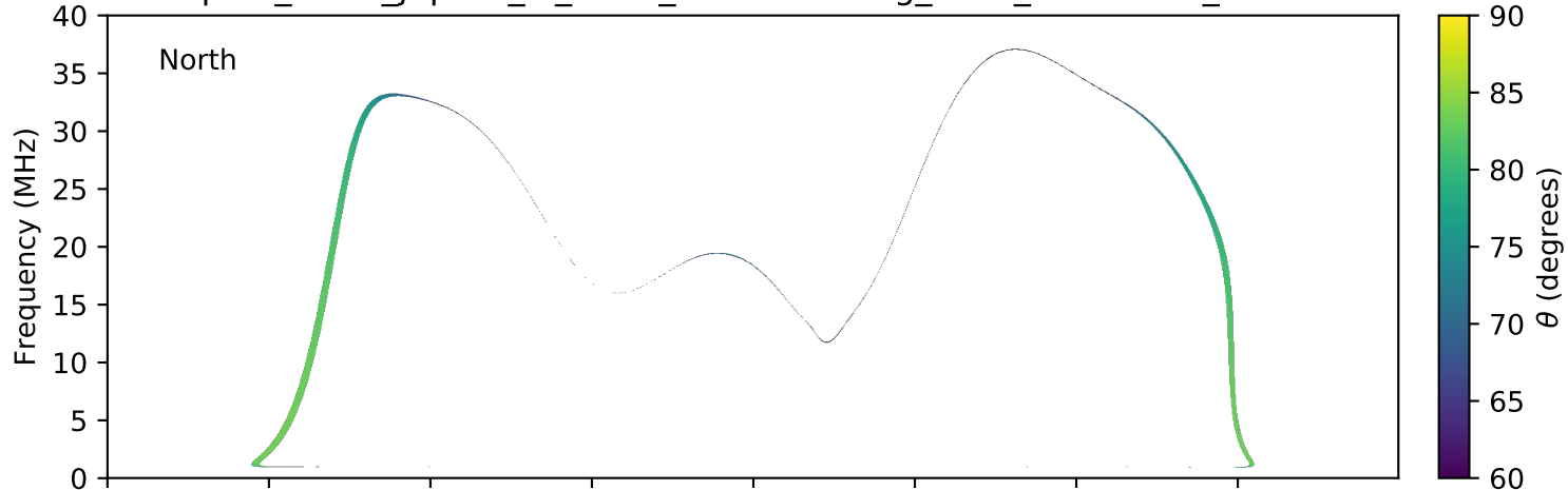
expres_earth_jupiter_io_isaac_lossc-wid1deg_3kev_20070408_v01.cdf
