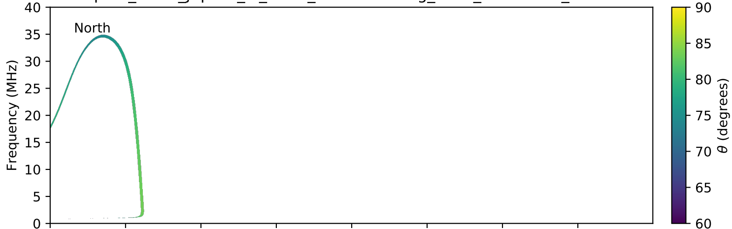
expres_earth_jupiter_io_isaac_lossc-wid1deg_3kev_20070407_v01.cdf
