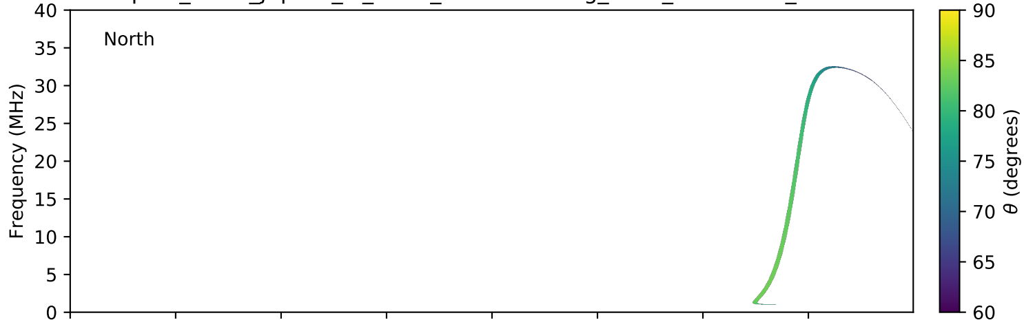
expres_earth_jupiter_io_isaac_lossc-wid1deg_3kev_20070402_v01.cdf
