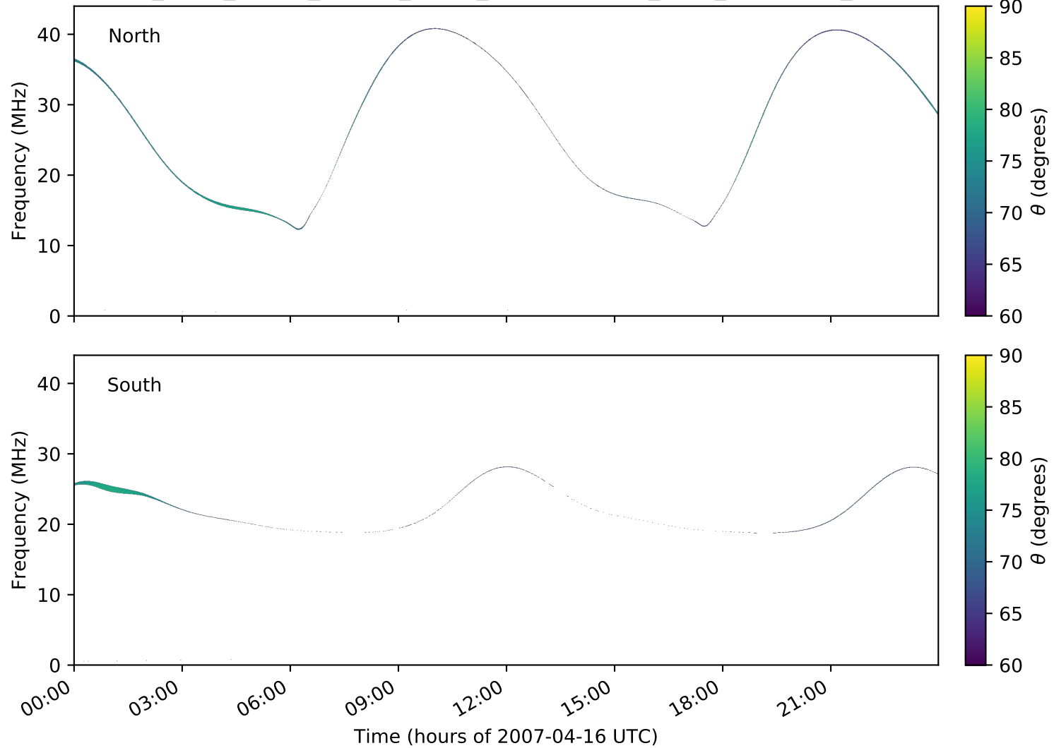
expres_earth_jupiter_europa_jrm09_lossc-wid1deg_3kev_20070416_v01.cdf
