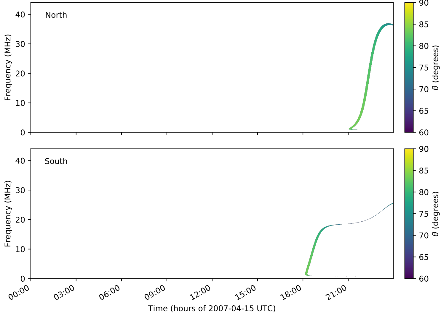
expres_earth_jupiter_europa_jrm09_lossc-wid1deg_3kev_20070415_v01.cdf
