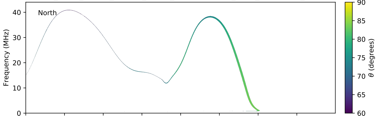
expres_earth_jupiter_europa_jrm09_lossc-wid1deg_3kev_20070413_v01.cdf
