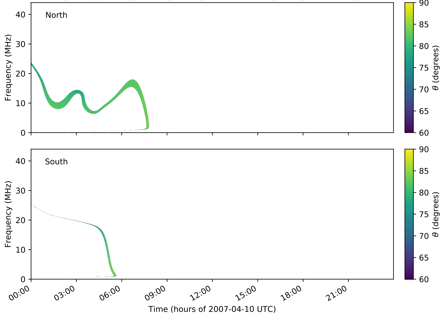
expres_earth_jupiter_europa_jrm09_lossc-wid1deg_3kev_20070410_v01.cdf
