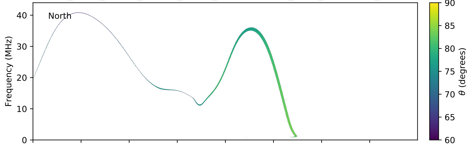
expres_earth_jupiter_europa_jrm09_lossc-wid1deg_3kev_20070406_v01.cdf
