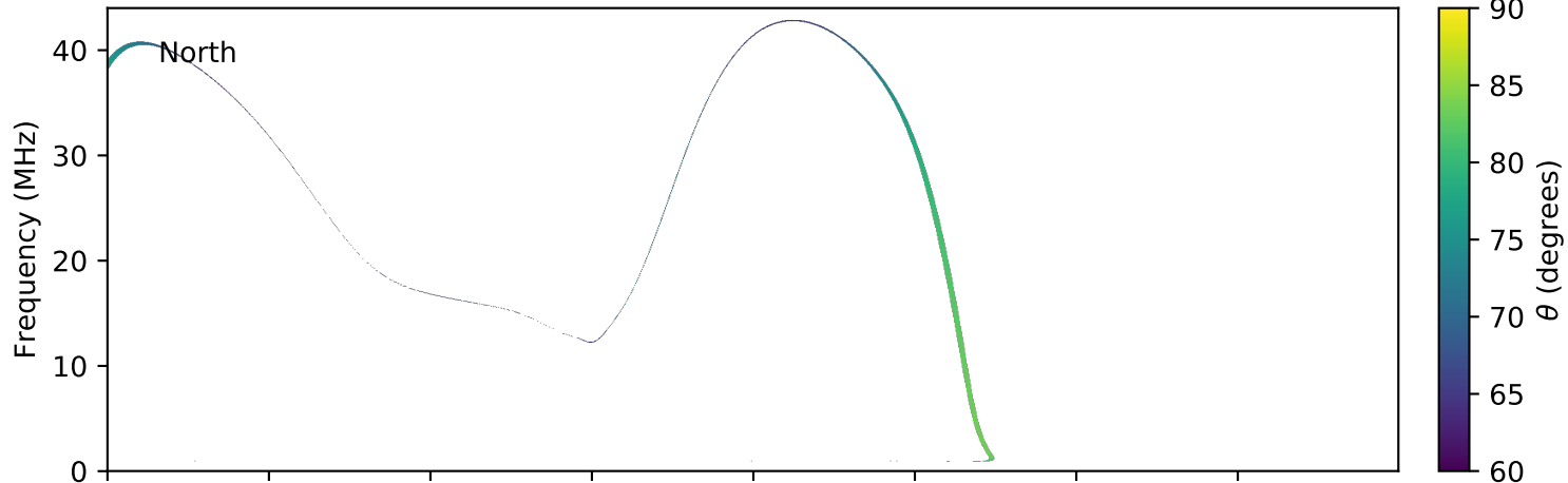
expres_earth_jupiter_io_jrm09_lossc-wid1deg_3kev_20070318_v01.cdf
