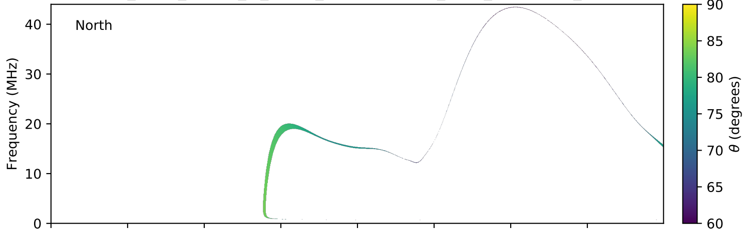
expres_earth_jupiter_io_jrm09_lossc-wid1deg_3kev_20070314_v01.cdf
