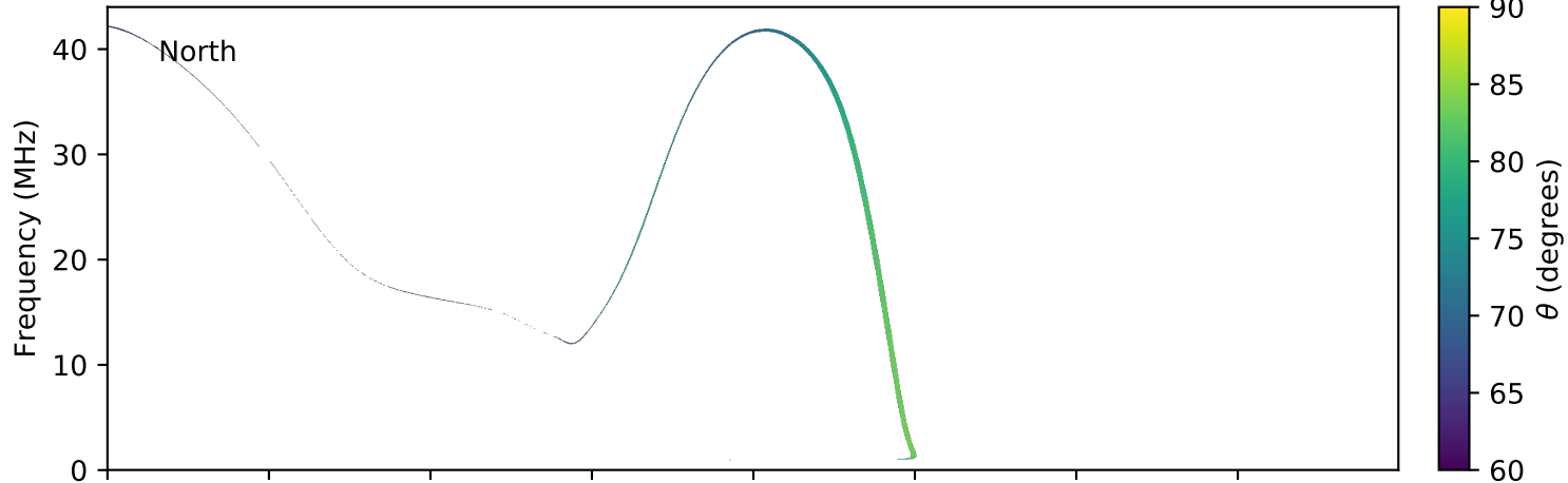
expres_earth_jupiter_io_jrm09_lossc-wid1deg_3kev_20070311_v01.cdf
