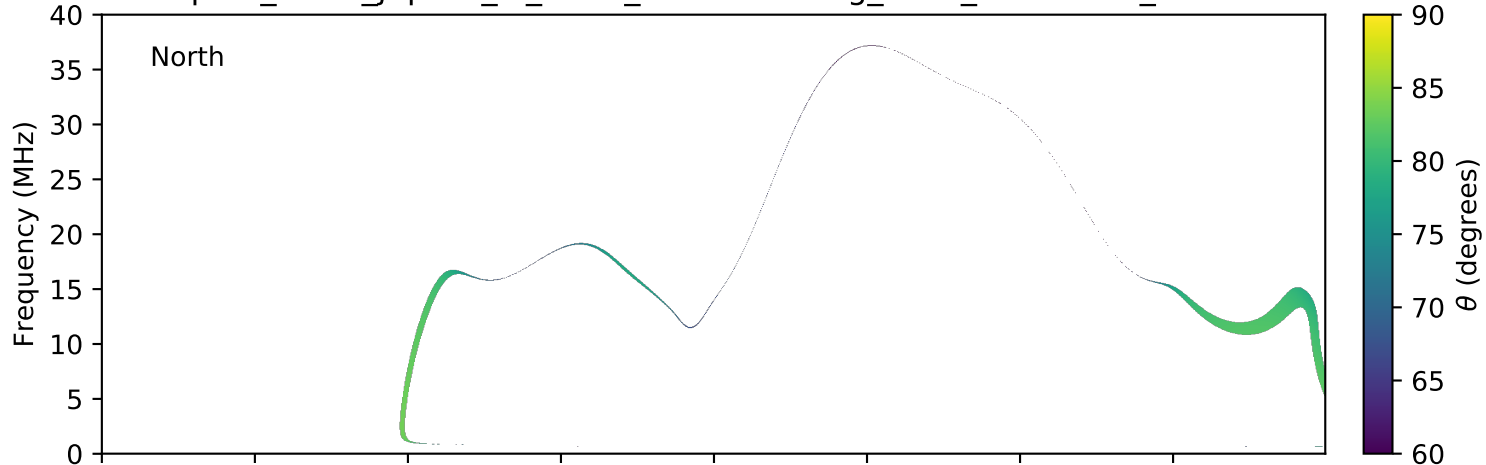
expres_earth_jupiter_io_isaac_lossc-wid1deg_3kev_20070330_v01.cdf
