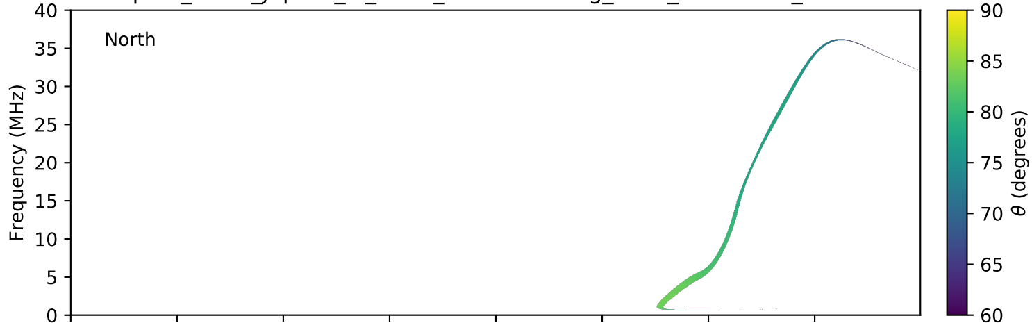
expres_earth_jupiter_io_isaac_lossc-wid1deg_3kev_20070326_v01.cdf
