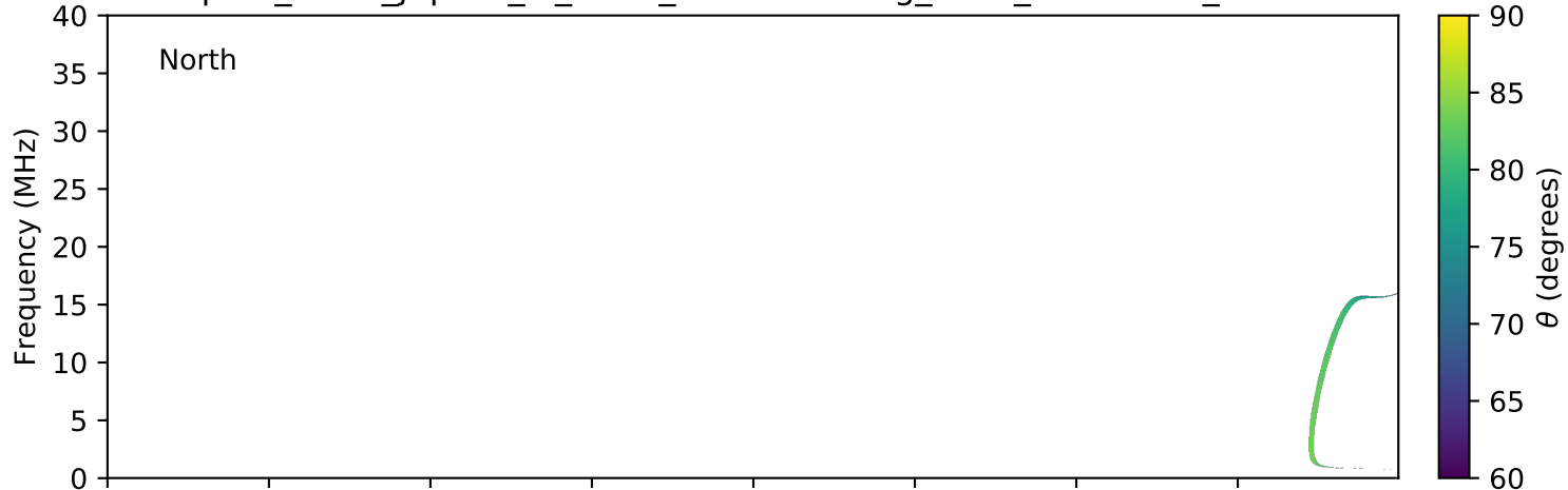
expres_earth_jupiter_io_isaac_lossc-wid1deg_3kev_20070324_v01.cdf
