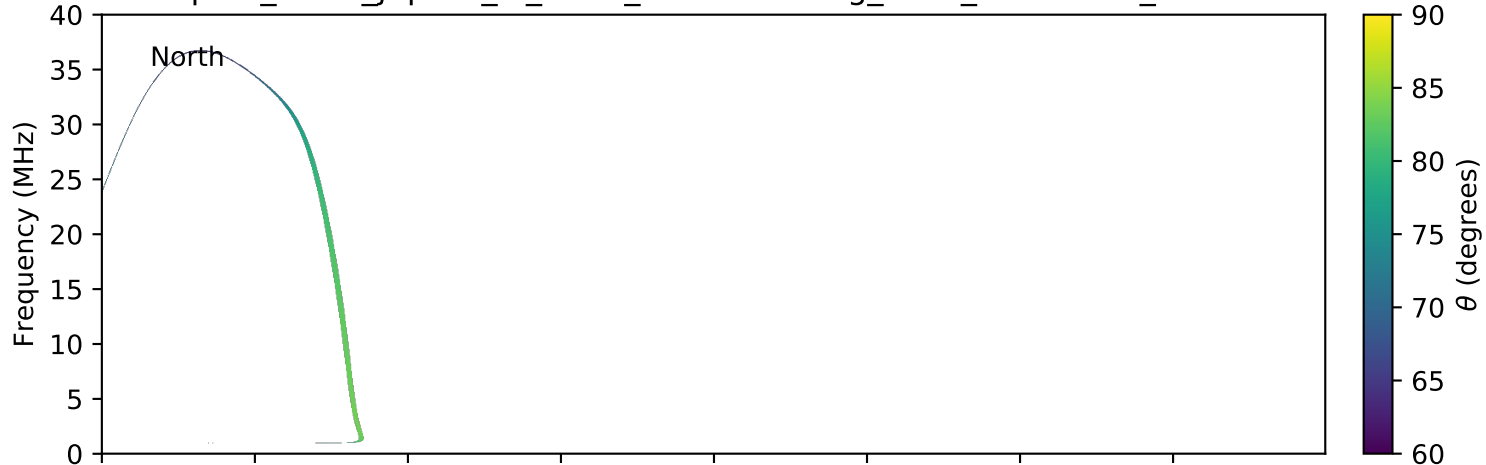
expres_earth_jupiter_io_isaac_lossc-wid1deg_3kev_20070322_v01.cdf
