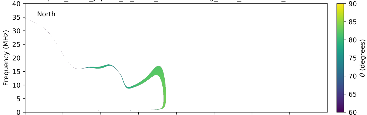
expres_earth_jupiter_io_isaac_lossc-wid1deg_3kev_20070320_v01.cdf
