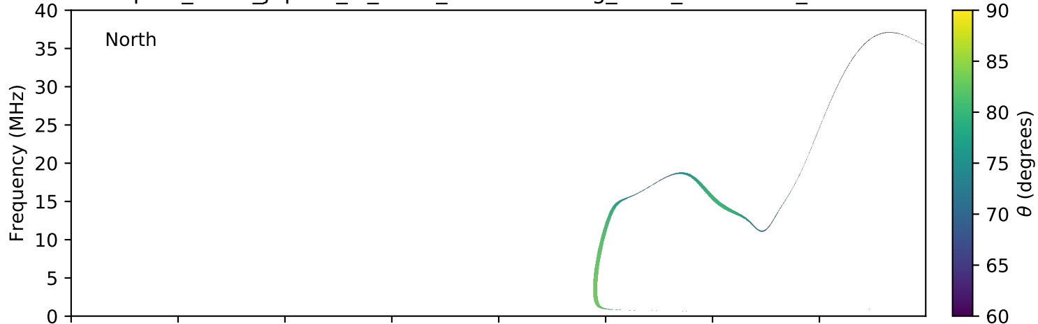
expres_earth_jupiter_io_isaac_lossc-wid1deg_3kev_20070319_v01.cdf
