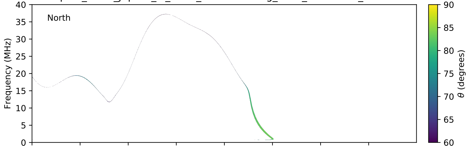
expres_earth_jupiter_io_isaac_lossc-wid1deg_3kev_20070318_v01.cdf
