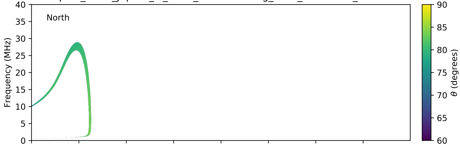
expres_earth_jupiter_io_isaac_lossc-wid1deg_3kev_20070315_v01.cdf
