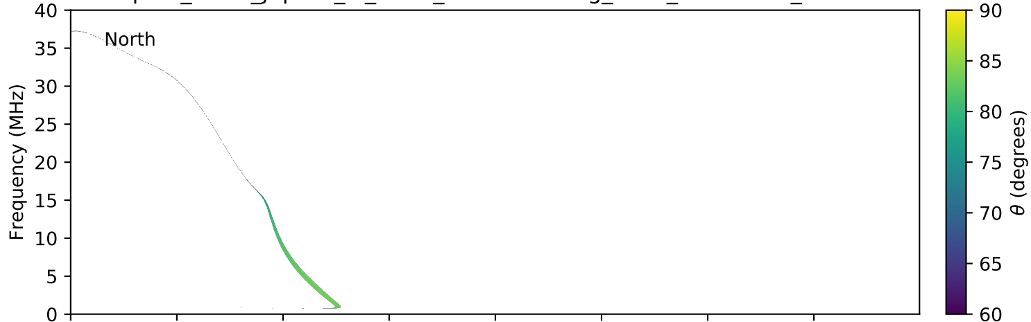
expres_earth_jupiter_io_isaac_lossc-wid1deg_3kev_20070313_v01.cdf
