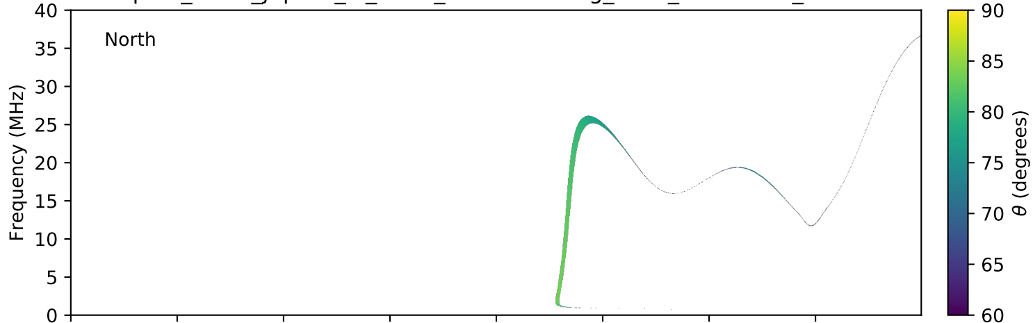
expres_earth_jupiter_io_isaac_lossc-wid1deg_3kev_20070312_v01.cdf
