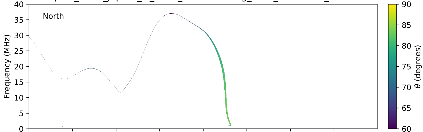
expres_earth_jupiter_io_isaac_lossc-wid1deg_3kev_20070311_v01.cdf
