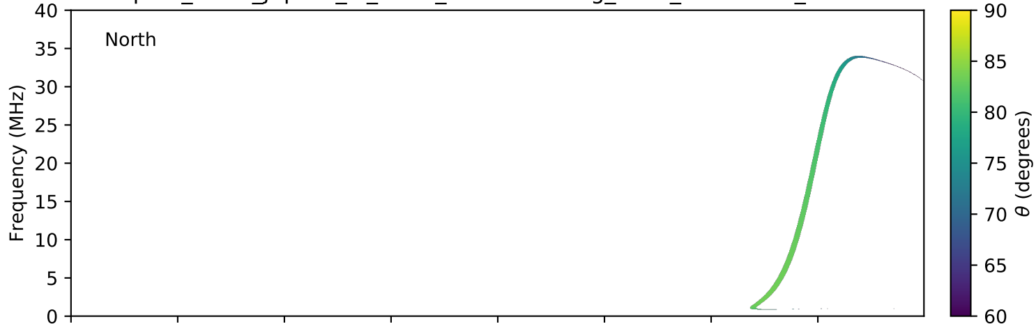
expres_earth_jupiter_io_isaac_lossc-wid1deg_3kev_20070310_v01.cdf
