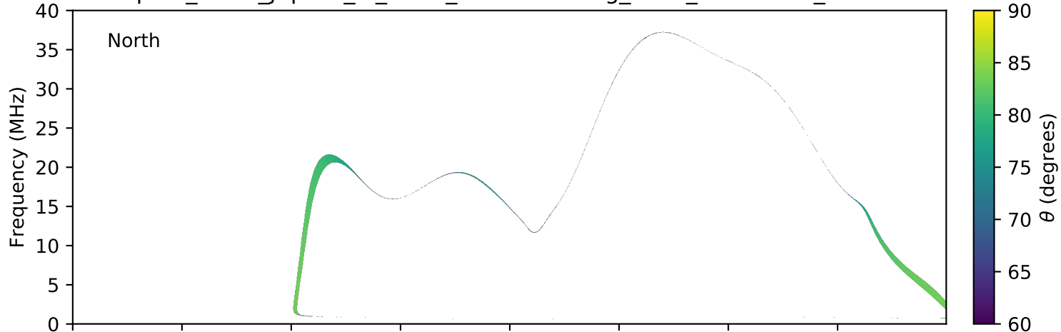
expres_earth_jupiter_io_isaac_lossc-wid1deg_3kev_20070307_v01.cdf
