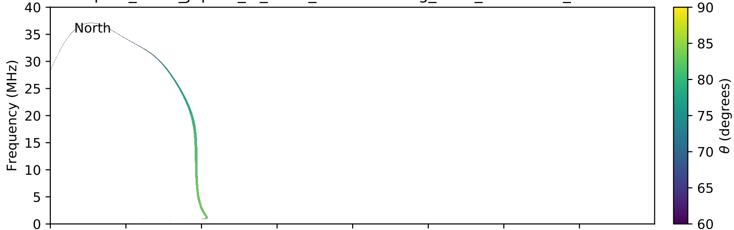
expres_earth_jupiter_io_isaac_lossc-wid1deg_3kev_20070306_v01.cdf
