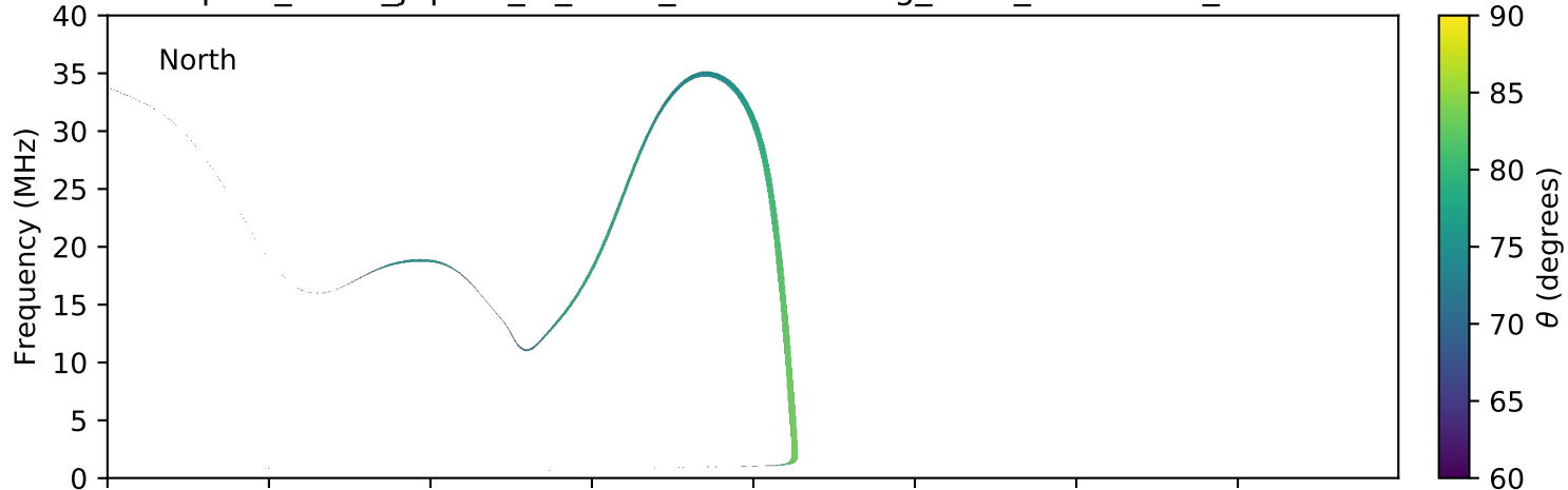
expres_earth_jupiter_io_isaac_lossc-wid1deg_3kev_20070304_v01.cdf
