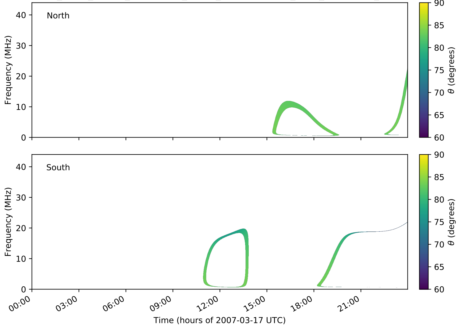
expres_earth_jupiter_ganymede_jrm09_lossc-wid1deg_3kev_20070317_v01.cdf
