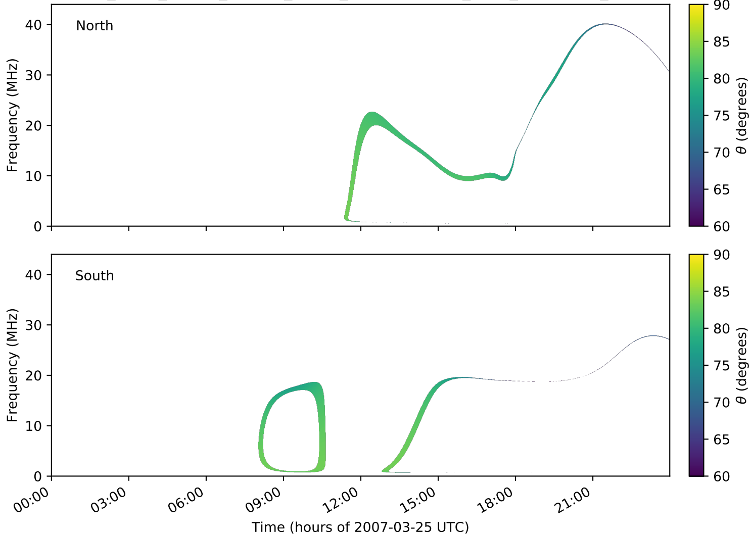
expres_earth_jupiter_europa_jrm09_lossc-wid1deg_3kev_20070325_v01.cdf
