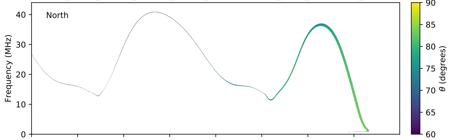
expres_earth_jupiter_europa_jrm09_lossc-wid1deg_3kev_20070319_v01.cdf
