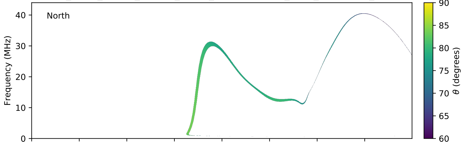
expres_earth_jupiter_europa_jrm09_lossc-wid1deg_3kev_20070318_v01.cdf
