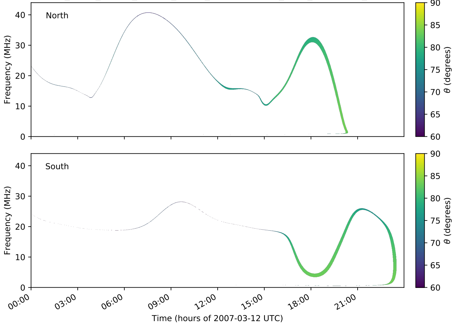
expres_earth_jupiter_europa_jrm09_lossc-wid1deg_3kev_20070312_v01.cdf
