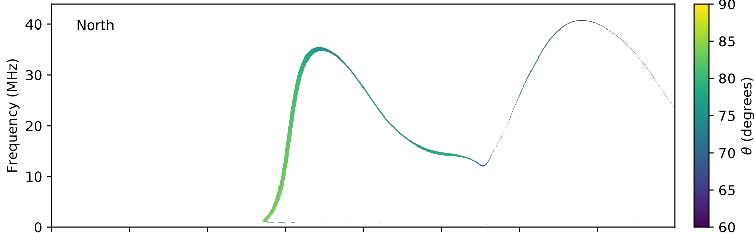
expres_earth_jupiter_europa_jrm09_lossc-wid1deg_3kev_20070311_v01.cdf
