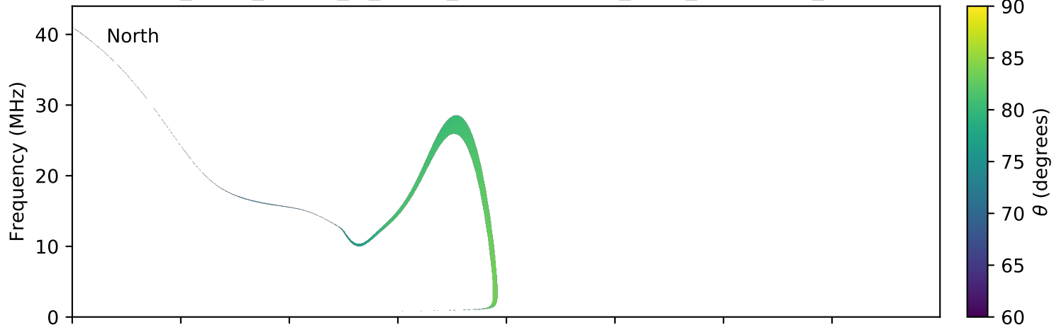
expres_earth_jupiter_io_jrm09_lossc-wid1deg_3kev_20070225_v01.cdf
