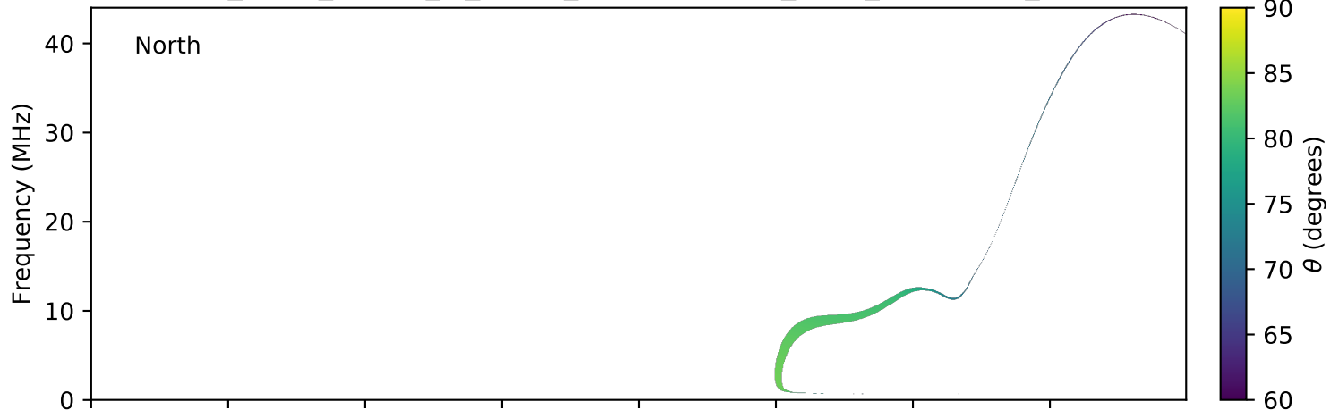
expres_earth_jupiter_io_jrm09_lossc-wid1deg_3kev_20070224_v01.cdf
