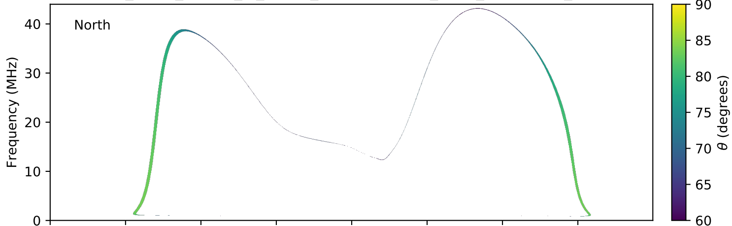
expres_earth_jupiter_io_jrm09_lossc-wid1deg_3kev_20070221_v01.cdf
