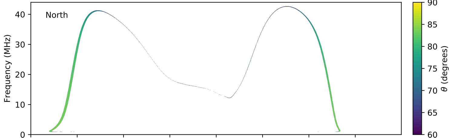
expres_earth_jupiter_io_jrm09_lossc-wid1deg_3kev_20070214_v01.cdf
