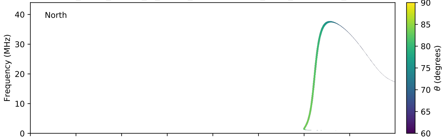
expres_earth_jupiter_io_jrm09_lossc-wid1deg_3kev_20070208_v01.cdf
