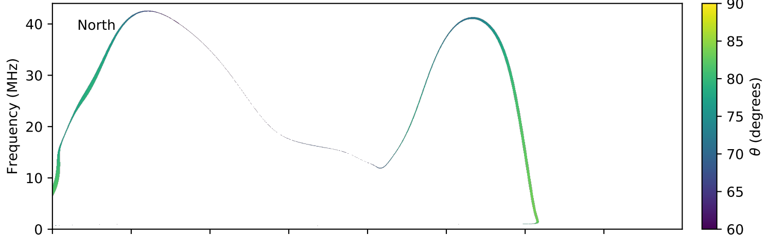
expres_earth_jupiter_io_jrm09_lossc-wid1deg_3kev_20070207_v01.cdf
