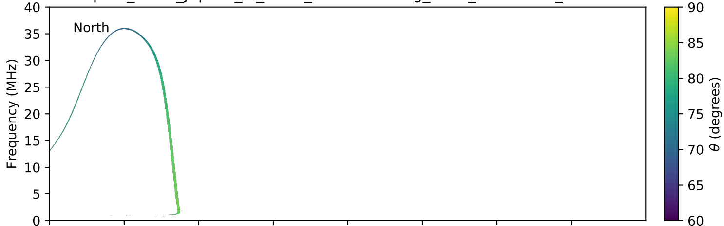
expres_earth_jupiter_io_isaac_lossc-wid1deg_3kev_20070227_v01.cdf
