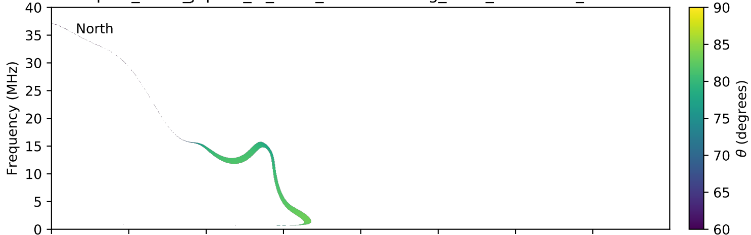
expres_earth_jupiter_io_isaac_lossc-wid1deg_3kev_20070225_v01.cdf
