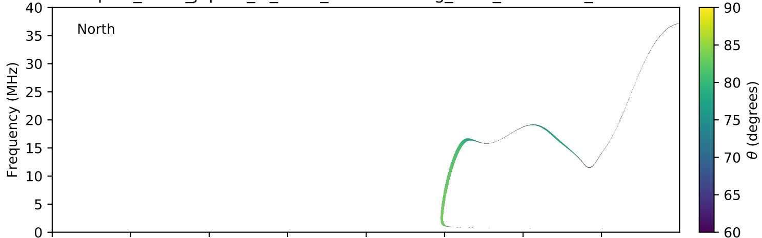
expres_earth_jupiter_io_isaac_lossc-wid1deg_3kev_20070224_v01.cdf
