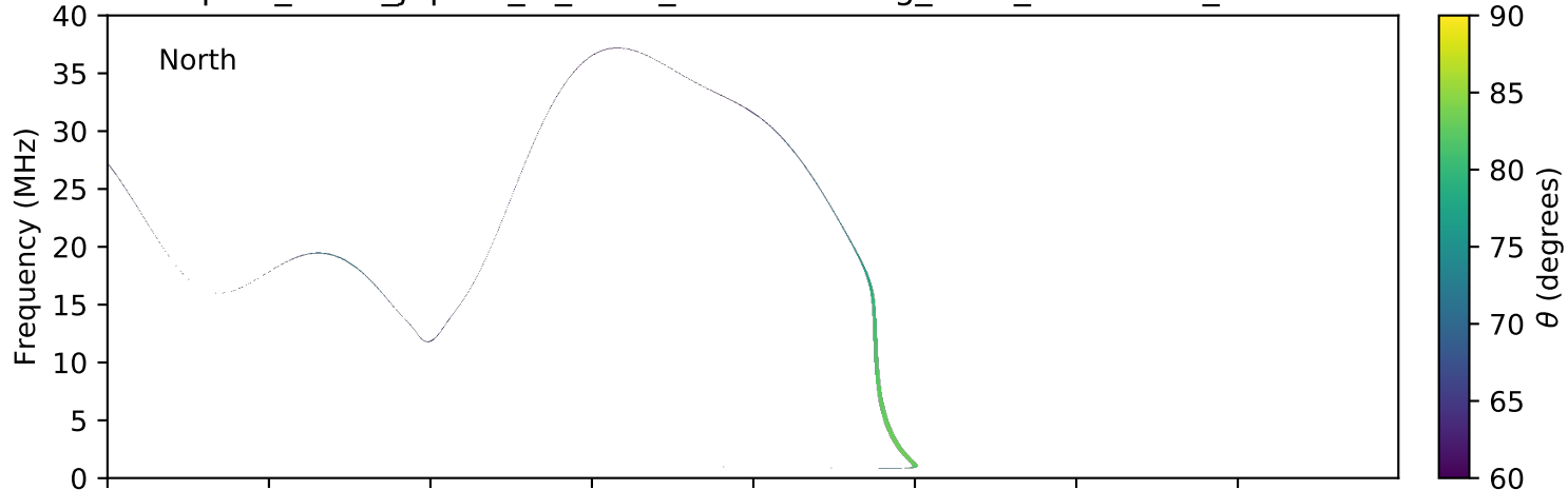
expres_earth_jupiter_io_isaac_lossc-wid1deg_3kev_20070223_v01.cdf
