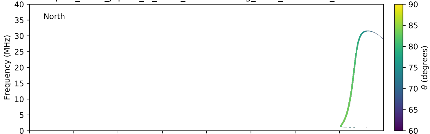
expres_earth_jupiter_io_isaac_lossc-wid1deg_3kev_20070222_v01.cdf
