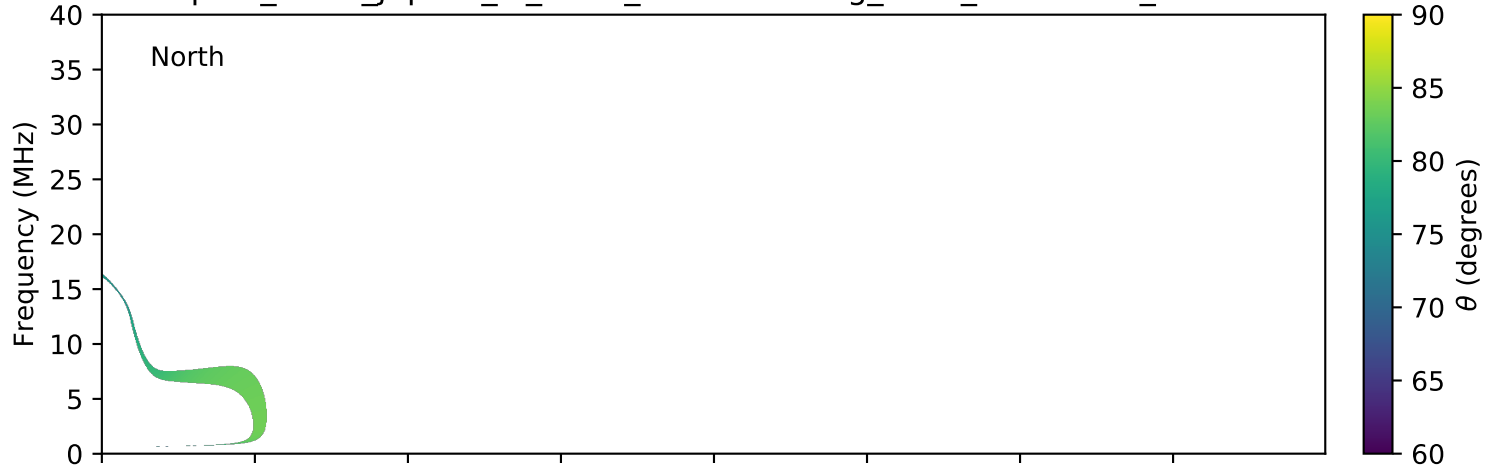
expres_earth_jupiter_io_isaac_lossc-wid1deg_3kev_20070220_v01.cdf
