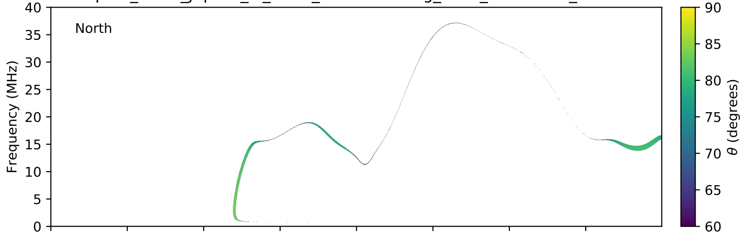
expres_earth_jupiter_io_isaac_lossc-wid1deg_3kev_20070219_v01.cdf
