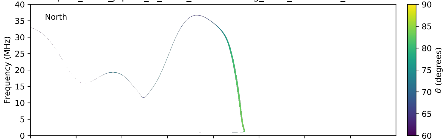
expres_earth_jupiter_io_isaac_lossc-wid1deg_3kev_20070216_v01.cdf
