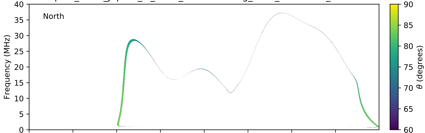
expres_earth_jupiter_io_isaac_lossc-wid1deg_3kev_20070212_v01.cdf
